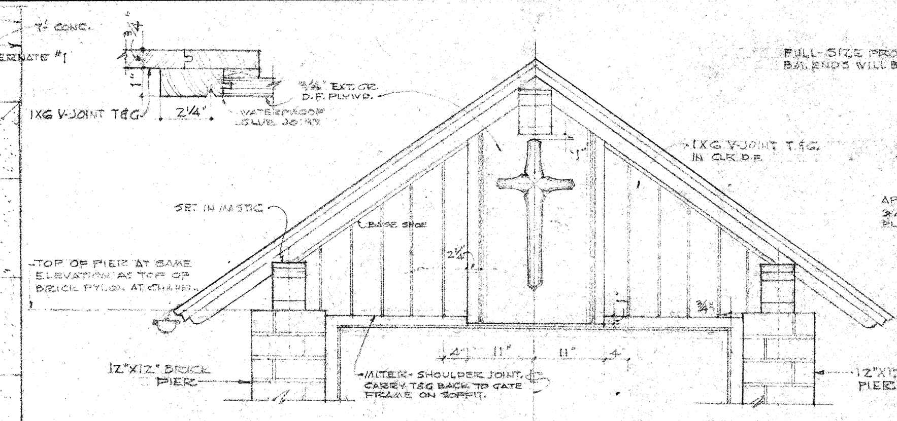
ELEVATION OF GABLE SCALE: 1/4" = 1'-0"
