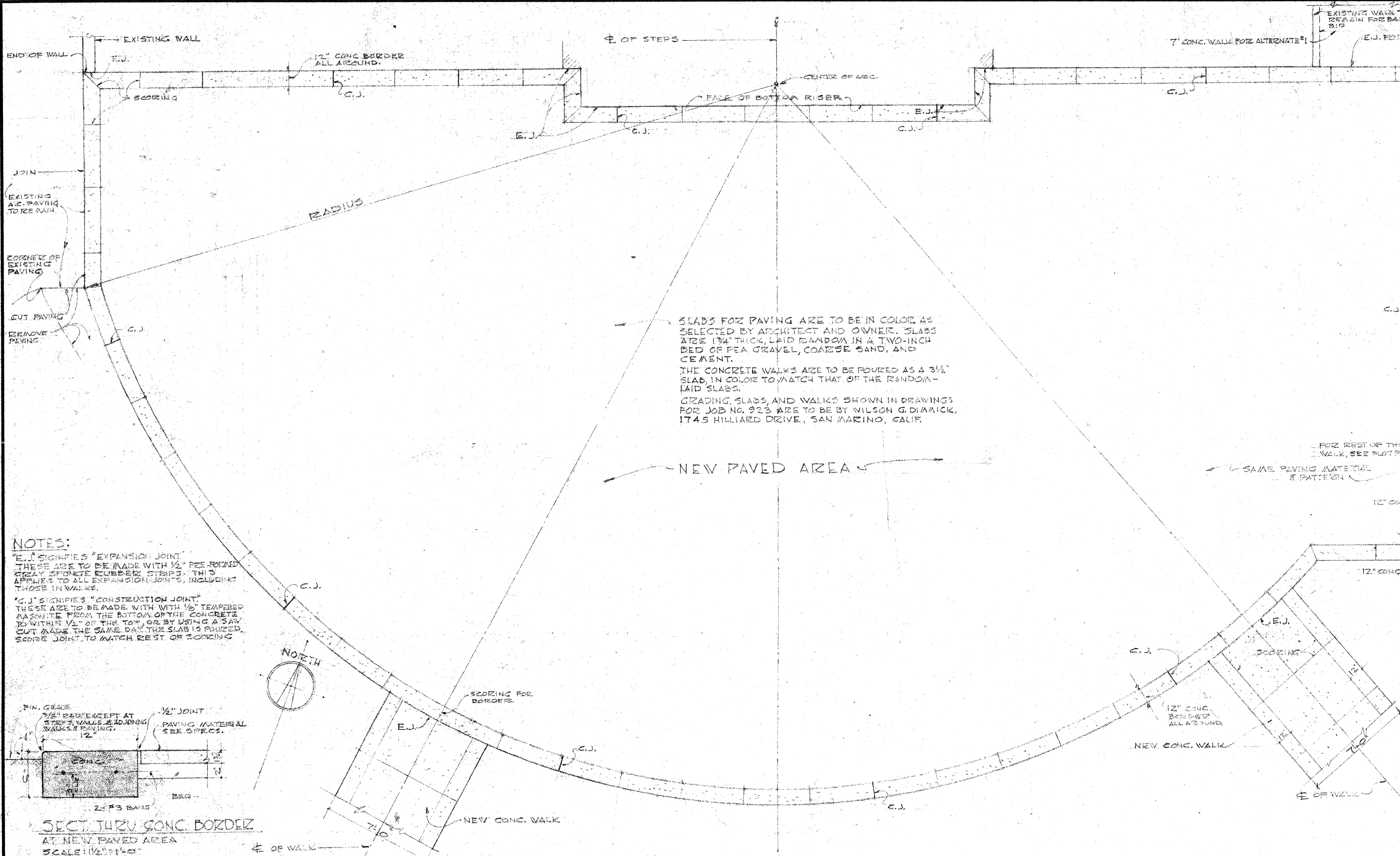
LAYOUT OF PAVED AREA... SCALE: 1/4" = 1'-0"
