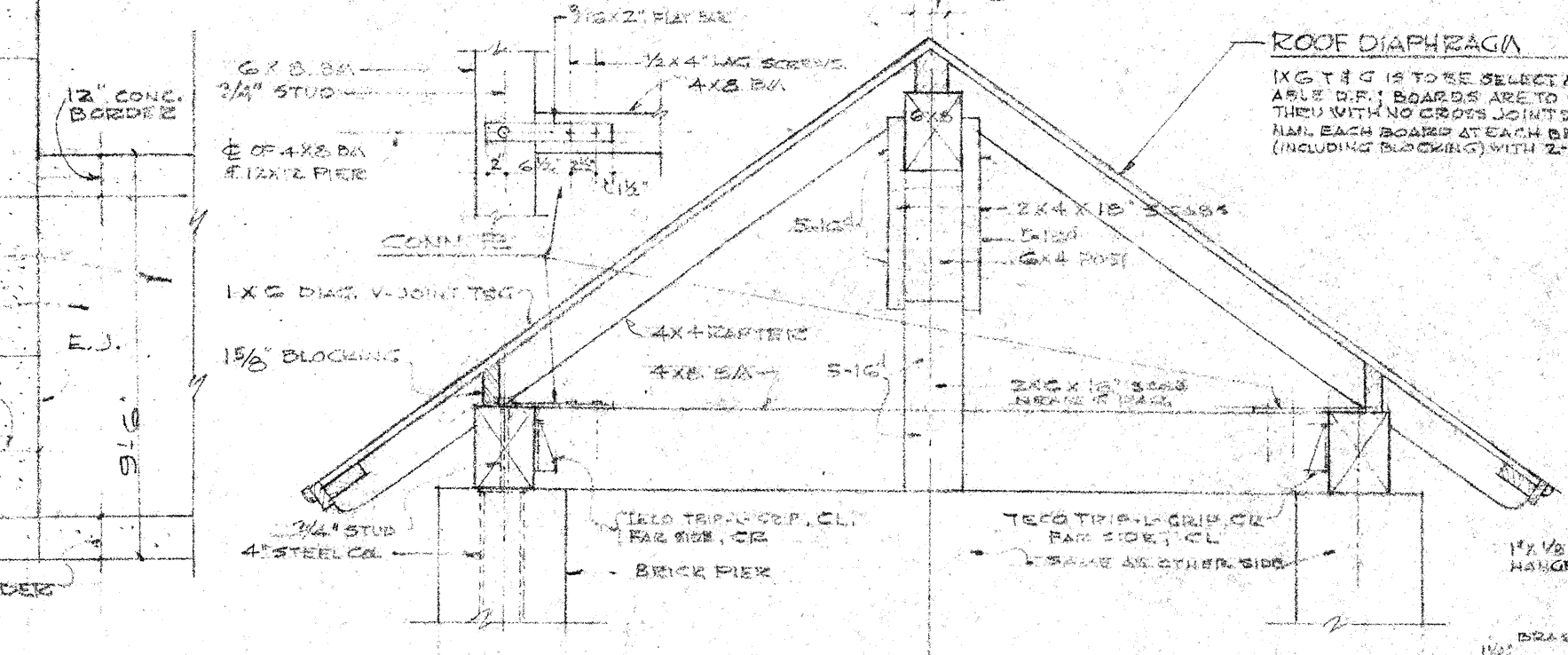
FRAMING AT F. OF BRICK PIERS SCALE: 1/4" = 1'-0"
