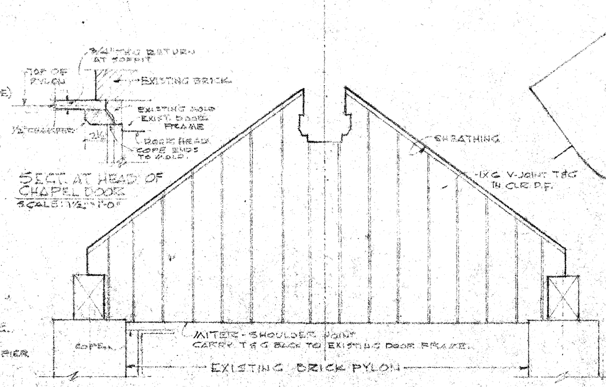
WOOD PANEL ABOVE CHAPEL DOOR SCALE: 1/4" = 1'-0"
