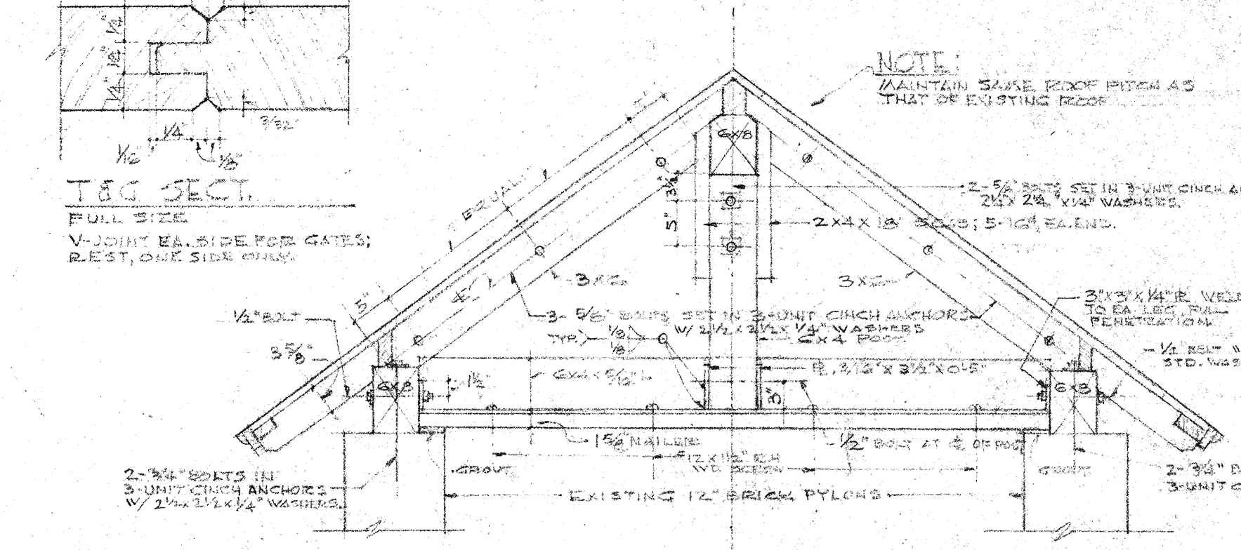
FRAMING AT FACE OF CHAPEL WALL SCALE: 1/4" = 1'-0"
