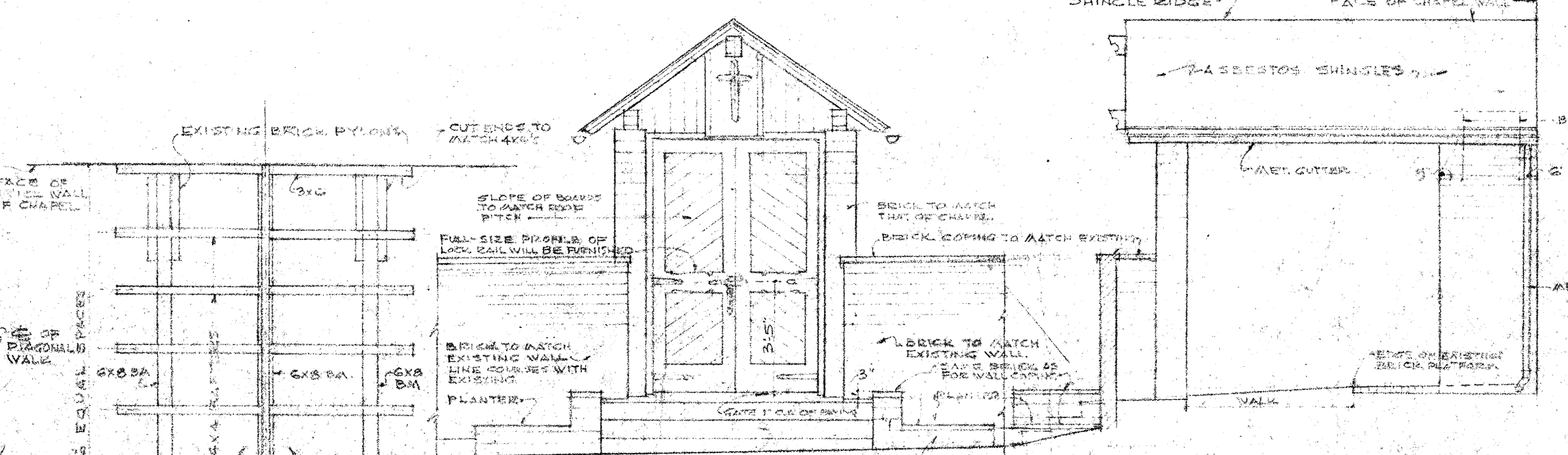
EAST ELEVATION
